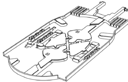
FOSC-AS-TRAY-S6/A6-1
